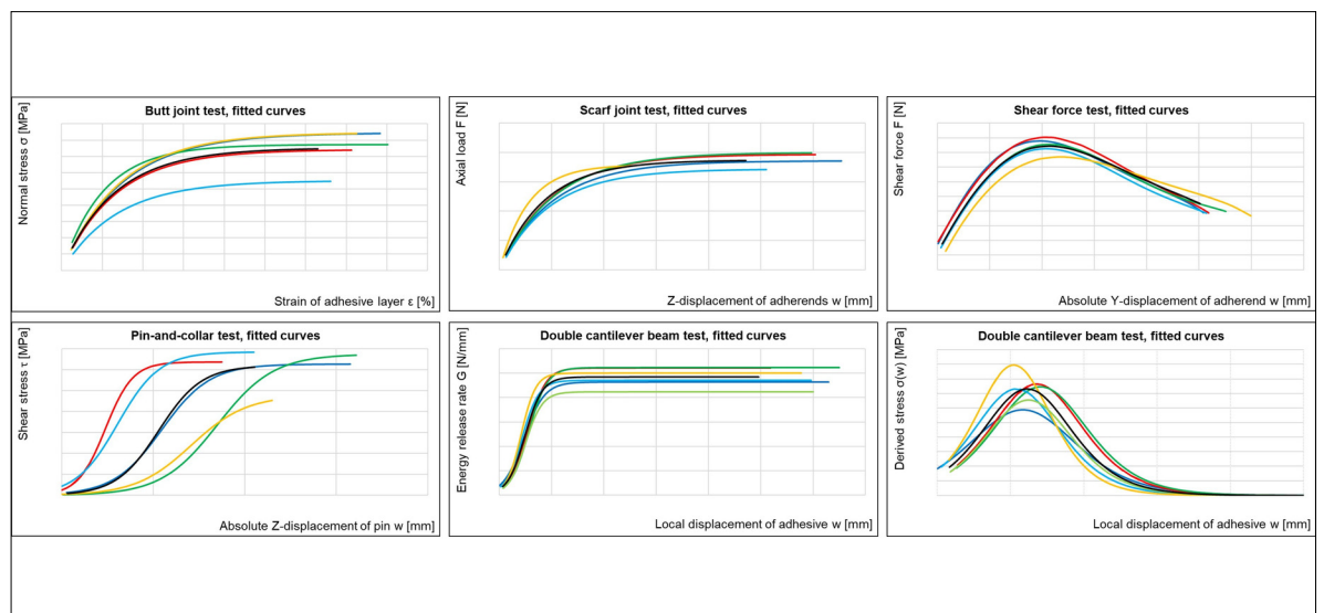
Reproducible experimental results representing the mechanical behaviour of the different bonded specimens
