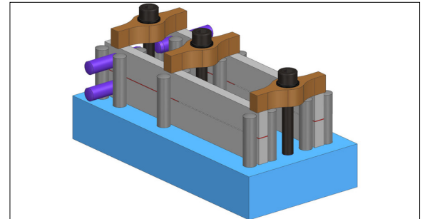
Multifunctional bonding and testing device for butt joint, scarf joint, shear and pin-and-collar tests.
