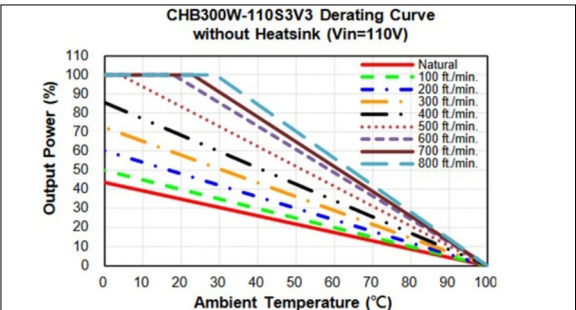
The derating curve illustrates how the PSU's output power decreases as the ambient temperature increases. Cincon, 2024
