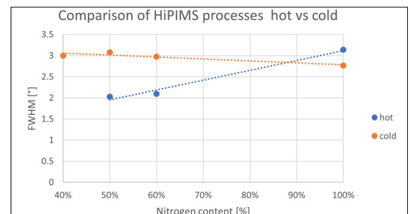
HiPIMS process dependence on the nitrogen content with substrate heating (blue) and without external heating (orange). Own presentation
