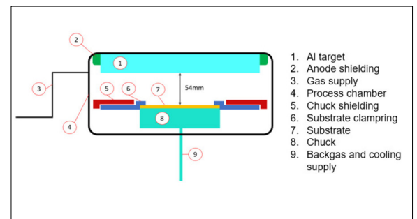
Cross-section of the utilized HiPIMS process module (CLUSTERLINE®200) showing the most important components. Own presentation
