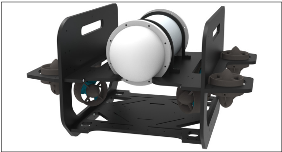
Underwater Robot Own presentation
