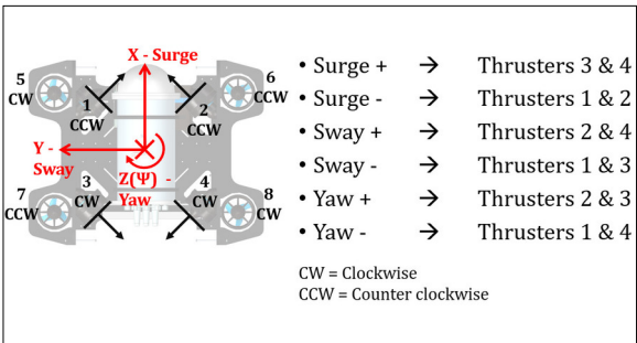
Thruster layout Own presentation
