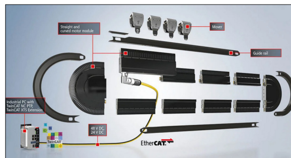
Abb. 1: Beckhoff XTS Beckhoff Automation
