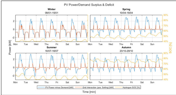
Seasonal diagram with the difference between produced and used power, interaction with electricity grid and hydrogen SOC Own presentment
