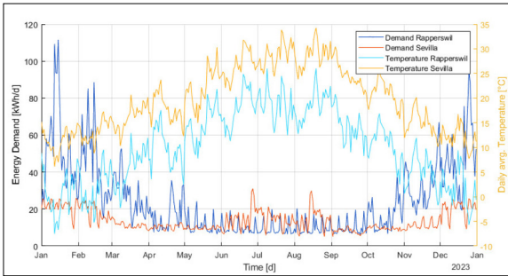
Daily Energy Demand of a two-person flat in Rapperswil and Sevilla over one year, including temperatures Own presentment
