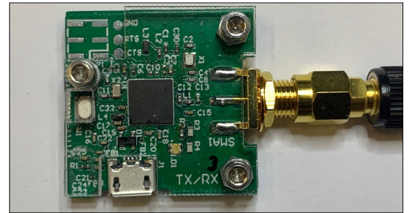
The designed hardware Own presentation
