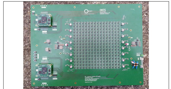
Levitation Board (16x16) Own presentation
