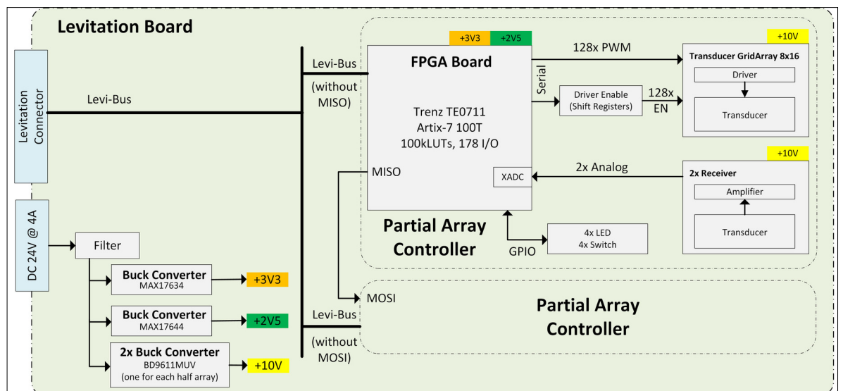
Block diagram of Levitation Board Own presentation
