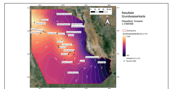
Figure 2: Map of the calculated groundwater potential in m a.s.l. Own presentation
