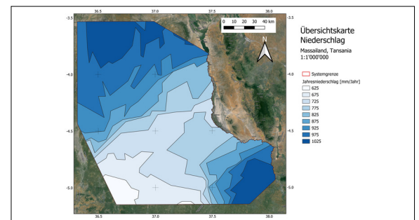
Figure 1: Overview map of annual precipitation in mm/year Own presentation
