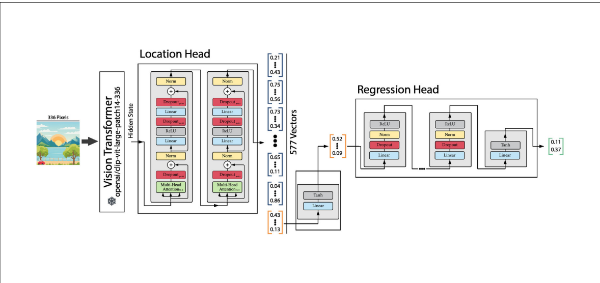
Regression Model Architecture Own presentment
