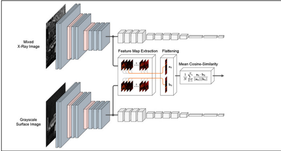
Coupled Dictionary Learning-Based Image Separation Network Own presentation
