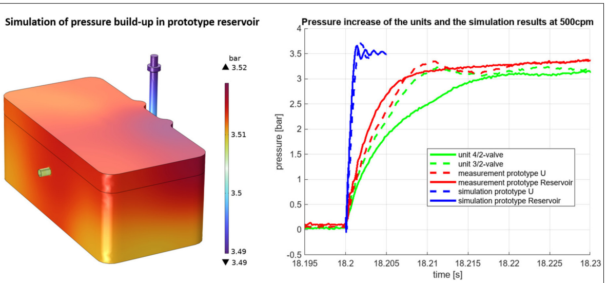
CFD simulation of the concept in COMSOL Multiphysics (left) and comparison between simulation and measurement (right) Own presentment
