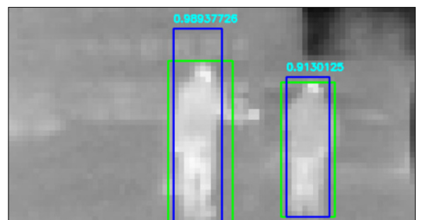
The network detects people in thermal images. Own presentment
