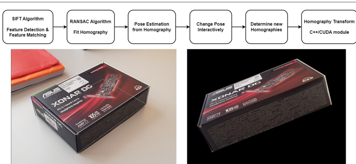
Mixed Python/C++/CUDA application: Input image with wireframe; Interactive real-time (5 ms) re-render in arbitrary pose. Own presentation
