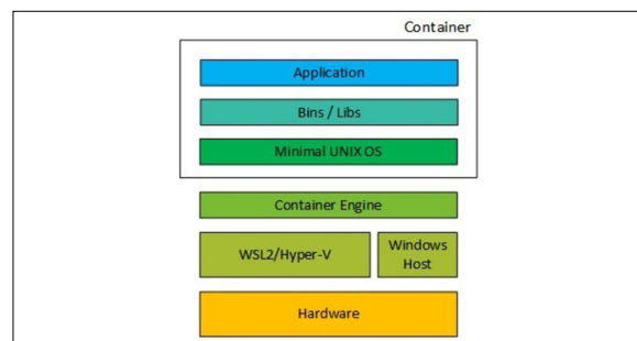
CV-DevContainer Toolchain. Own presentation
