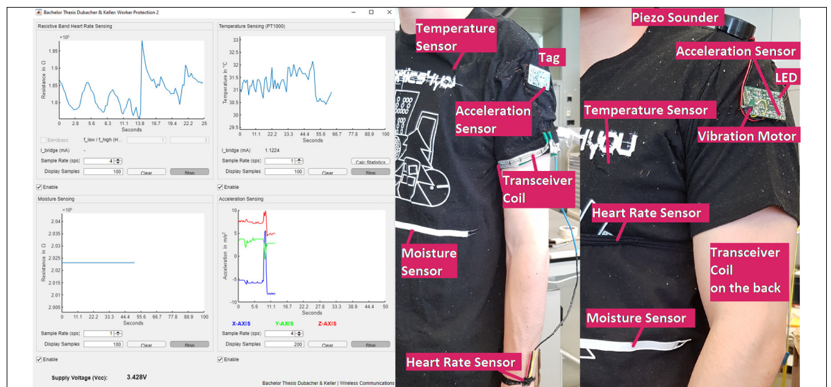
Demonstration setup with software on the left and textile-based hardware on the right used for worker protection. Own presentation
