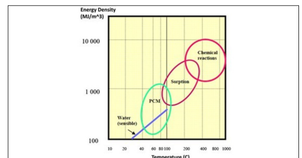
Energy densities of different thermal energy storage methods N'Tsoukpoe et al., 2009
