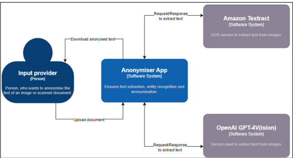
C4 Context diagram of the Anonymiser App. Own presentation
