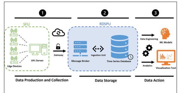
Fig. 1: Schematic of an energy plant monitoring data pipeline with a remote time series database. Own presentation
