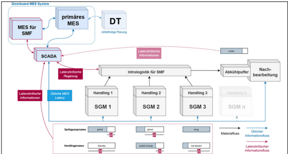
Figure 3: Digital system architecture for application with Seamless Material Flow integration.
