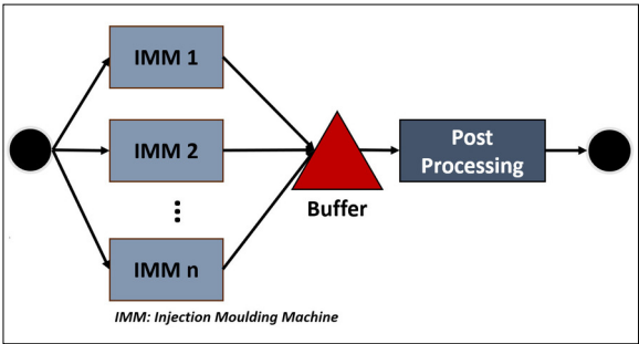
Figure 1: Use case in discrete manufacturing: injection moulding to buffer to cutting and packaging.
