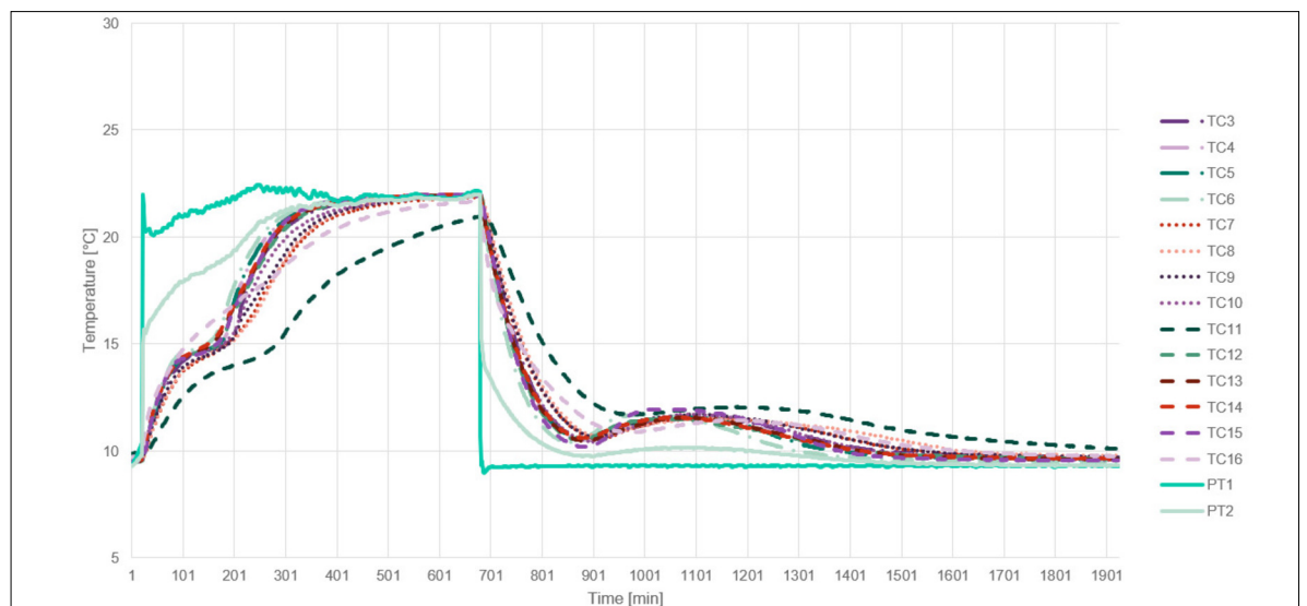
Temperature curve of PCM test cycle 2 Own presentation
