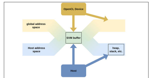
Representation of the address space of a SVM Buffer
