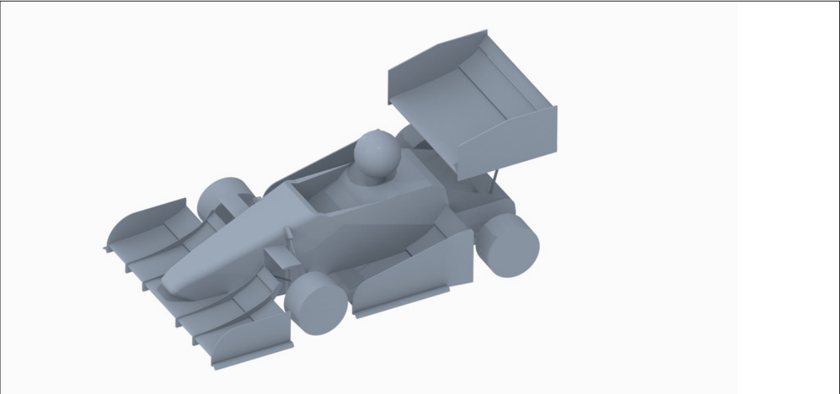
Overall model of the concept of a possible aero package with high downforce. Own presentment
