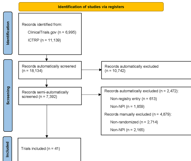
Figure 1 Retrieval and trial selection process. Abbreviations: ICRP, International Clinical Trials Registry Platform; NPI, non-pharmaceutical interventions.
