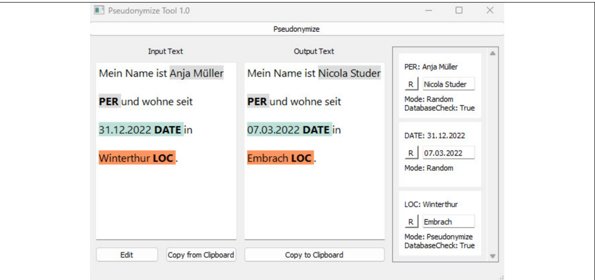
Pseudonymize Tool 1.0 Graphical User Interface Own presentation
