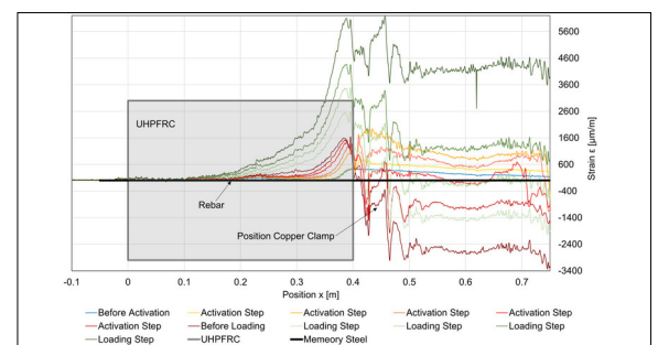
Fig. 2: Postprocessing of the fibre optical strain measurements of a pull-out test with long embedment length Own presentation
