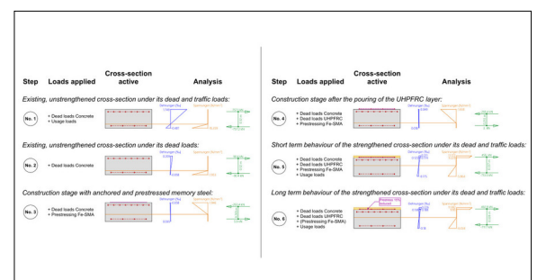
Fig. 3: The construction stages of the UHPFRC and memory steel strengthening system during the rehabilitation Own presentation
