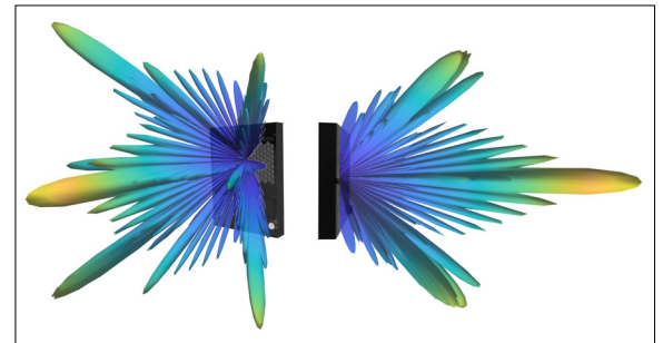
Beam Radiation Pattern Own presentation
