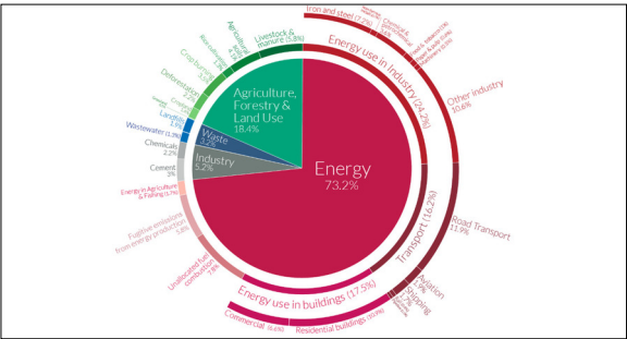
Global CO 2 emissions by sector (2016). https://ourworldindata.org/ghg-emissions-by-sector
