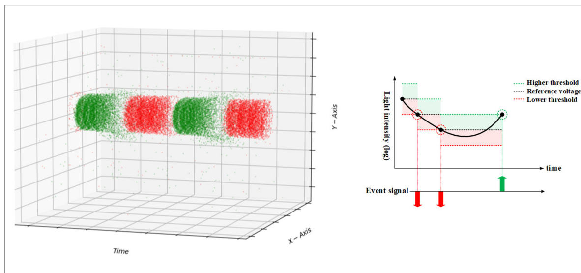
Point cloud of events generated from a flashing LED and visualization of event generation on the sensor. Own presentation
