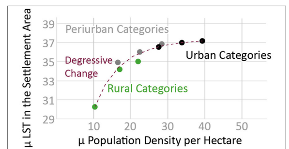
Fig. 3: Correlation Analysis between average Population Density and average LST of the nine Municipal Categories. Own presentment 2023; NASA and USGS 2022; swisstopo 2022
