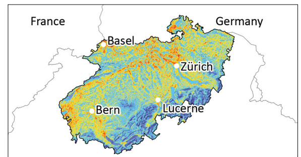
Fig. 1: Study Perimeter in German-speaking Switzerland with the GIS generated Land Surface Temperature (LST). Own presentment 2023; NASA and USGS 2022; swisstopo 2022
