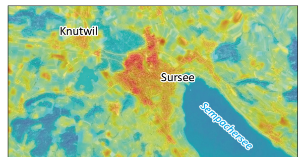
Fig 2: The Degree of Heat Stress in the small City Sursee is higher than in the rural Environment. Own presentment 2023
