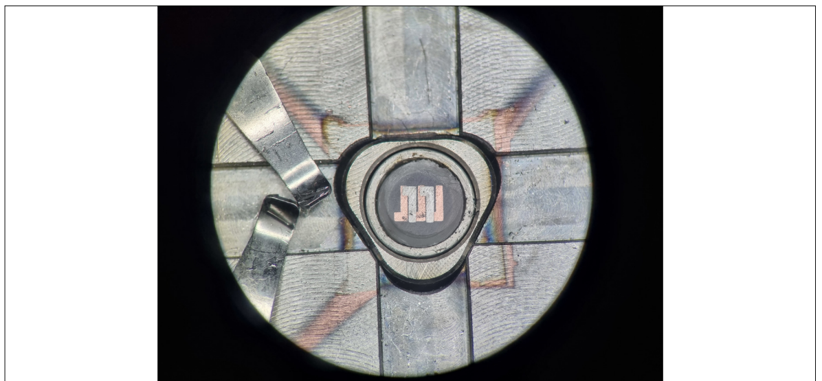
Fig 3: Microscopic picture of a type T thermocouple deposited on a POM substrate. Length 1.2mm, film thickness 80nm. Own presentment
