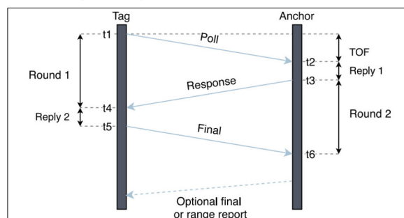
Double-sided two-way-ranging (TOF: Time of Flight, [t1, ..., t6]: timestamps). https://doi.org/10.1016/j.adhoc.2021.102637
