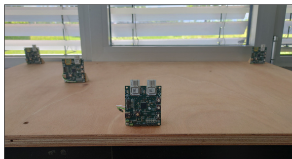
Radio beacon modules deployed in a test setup. Own presentation
