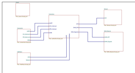
Schematic block diagram of the designed radio beacon modules. Own presentation
