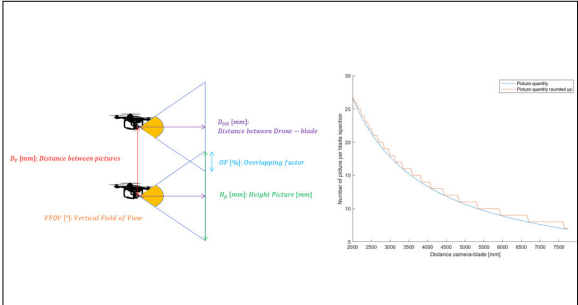
Determination of the maximal drone-blade distance for a defined minimal image quality. Own presentation
