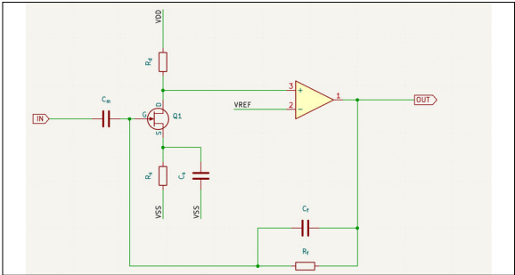
Charge Sensitive Amplifier with JFET Preamplifier Own presentment
