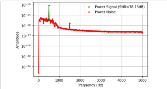
ELIA Output Spectrum from transient noise SPICE simulation, 71 PPM variation Own presentment
