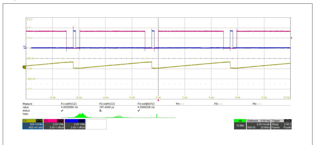
Figure 3. Output of the charge amplifier (C1), integration phase (C2) and reset phase (C3). Own presentment
