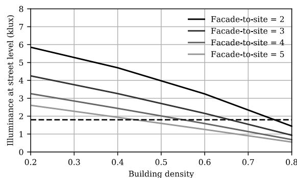
Fig. 2. Illuminance at street level for different urban densification parameters of an urban site (neighbourhood, town). Urban densification parameters are 1) the building density, defined as the ratio between the building footprint and the total horizontal area of the urban site, and 2) the façade-to-site ratio, defined as the ratio between the area of all vertical surfaces in the urban site and the total horizontal area of the urban site. For each combination of building density and façade-to-site ratio, the graph provides the illuminance at street level, assuming a CIE overcast sky at 12:00 LT on the 21st of March in Zürich. The underlying simulations have been carried out with the raytracing tool “Radiance”. The dashed line indicates that certain combinations of building density and facade-to-site ratios lead to scenarios where a minimum threshold of 1800 lux of daylight for circadian entrainment is not guaranteed for the given time.
