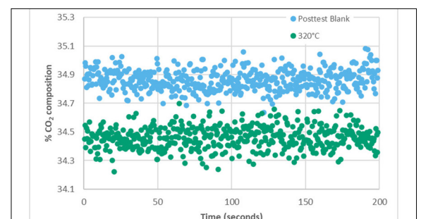
Carbon dioxide removal by liquid metal from a CO 2 -Argon gas stream in a laboratory bubble column reactor Own presentment
